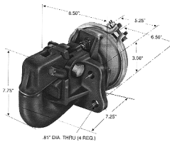
Less plunger, air cylinder, & bracket 1. HOLPH-200-1
