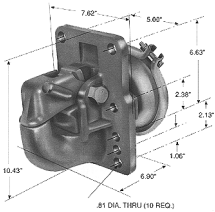
Less plunger, air cylinder, bracket
